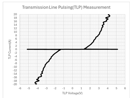
Figure 4. TLP(1/100nS)
